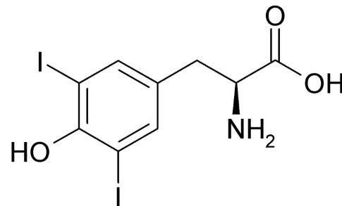
Image 6: Diiodotyrosine (T2) 12
