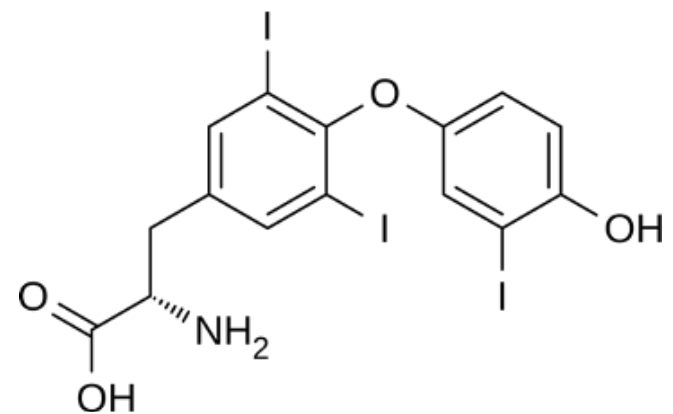
Image 4: Triiodothyronine (T 3 )
