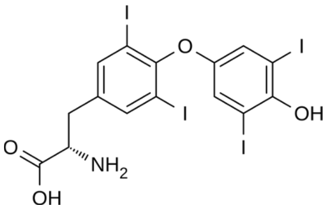
Image 3: Thyroxine (T 4 ) 4
